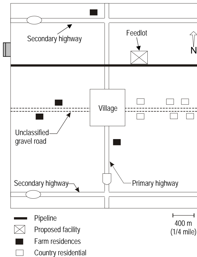
Figure 5 - Area sketch for example 1
